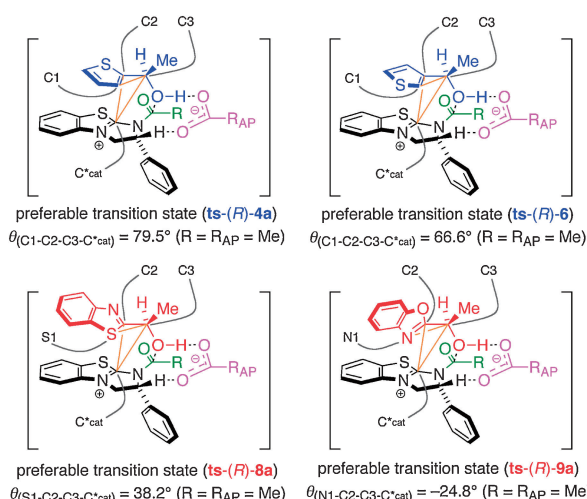
Figure 2. Transition structures ts-(R)-4a , ts-(R)-6 , ts-(R)-8a , and ts-(R)-9a derived from ( R )-1-(2-thienyl)ethanol (( R )-4a), ( R )-1-(3-thienyl)ethanol (( R )-6), ( R )-1-(benzothiazol-2-yl)ethanol (( R )-8a), and ( R )-1-(benzoxazol-2-yl)ethanol (( R )-9a) with the intermediary zwitterionic species ( int-II ).
