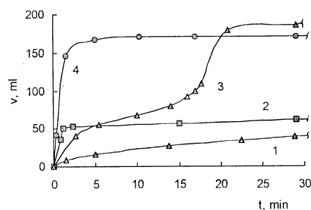
Fig. 2. Time dependencies of the volume of generated gas in the reaction of \text{EtAlCl}_2 (0.65 M) in toluene (40 °C): (1) with 1 (0.54 mmol); (2) with TBP (0.16 M); (3) with 1 (0.54 mmol) + TBP (0.16 M); (4) with 1 (0.54 mmol) and TBP (0.16 M) in the presence of HCl (0.3 M).
