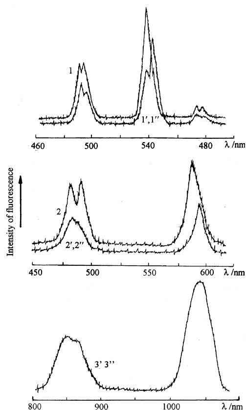
Fig. 3. Luminescence spectra (298 K): 1, 2 — \text{LnCl}_3 \cdot 6\text{H}_2\text{O} , Ln = Tb ( 1 ), Dy ( 2 ); the emission from \text{NdCl}_3 \cdot 6\text{H}_2\text{O} was too weak to be detected. 1', 2', 3' and 1'', 2'', 3'' — the solutions of \text{LnCl}_3 \cdot 3\text{TBP} complexes and the solutions after reactions of \text{LnCl}_3 \cdot 6\text{H}_2\text{O} (6.48 mmol) with \text{Et}_3\text{Al} (0.54 mmol) in toluene at \text{TBP}/\text{Ln} \geq 12:1 ; Ln = Tb ( 1', 1'' ), Dy ( 2', 2'' ), Nd ( 3', 3'' ). \lambda_{\text{excitation}} (nm) = 365 ( 1, 1', 1'' ), 352 ( 2, 2', 2'' ), 337, 1 ( 3', 3'' ).
