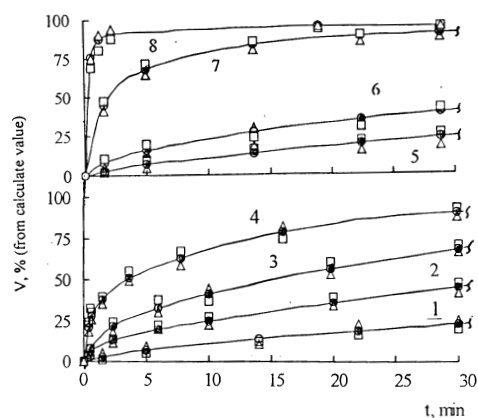
Fig. 1. Time dependencies of the volume of generated gas in the reaction of 1–3 (0.54 mmol) with R_n\text{AlX}_{3-n} (6.5 mmol) in toluene: 1–4 at interaction of 1–3 with \text{Et}_3\text{Al} without TBP: (1) 40 °C, (2) 50 °C, (3) 70 °C, (4) 90 °C; 5–8 at interaction (40 °C) of 1–3 with \text{Et}_3\text{Al} , \text{Et}_2\text{AlCl} , (i\text{-Bu})_3\text{Al} , \text{EtAlCl}_2 , respectively, without TBP; –○– Tb, –□– Dy, –△– Nd.
