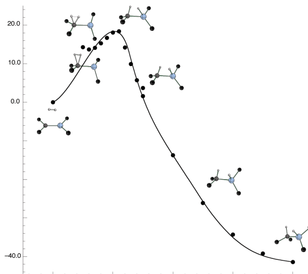
Figure 5. Computed reaction profile (ONIOM(MPW1K/6-311++G-(d,p))) for \text{H}_2 addition/dissociation (energies are given in kcal/mol).
