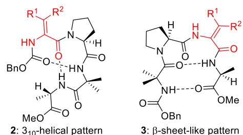
Figure 3. 3 10 -Helical and β-sheet-like conformations.
