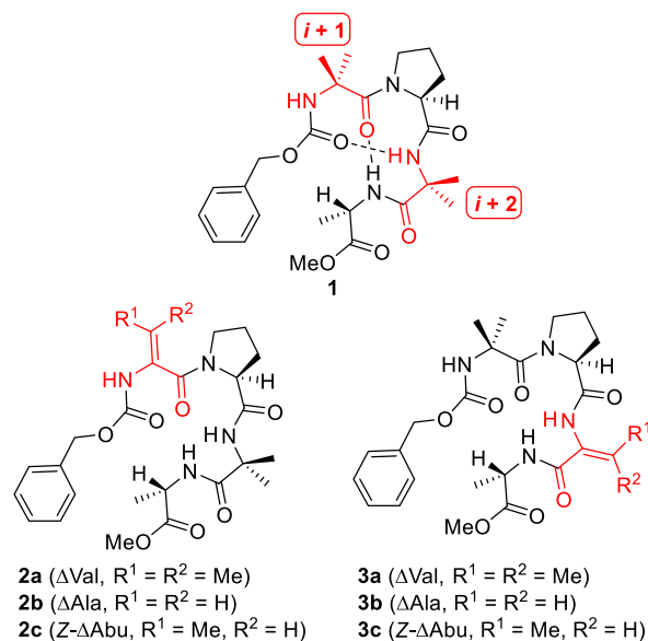
Figure 2. Balaram's incipient 3_{10} helical peptide ( 1 ) and proposed \Delta\text{AA} -containing variants ( 2 and 3 ).
