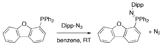
Scheme 1. Synthesis of Ligand L
