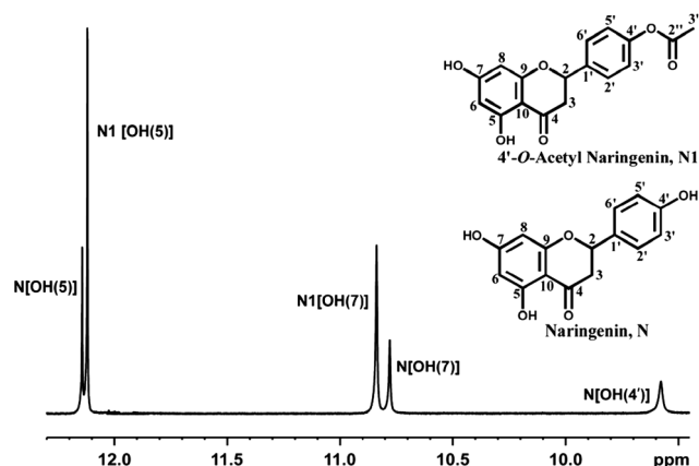
Fig. 4 OH region of the 500 MHz ^1\text{H} NMR spectrum recorded of the crude reaction products of the enzymatically obtained monoacylated derivative of naringenin (2.30 \mu\text{mol} ) in \text{DMSO}-d_6 . Assignments of the resonances of the unreacted naringenin (N) and the monoacylated product (N1) are denoted.
