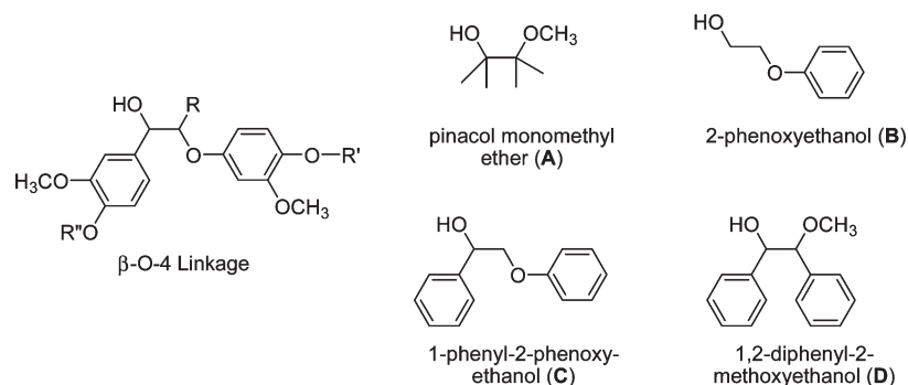
Figure 1. \beta -O-4 linkage and lignin model complexes.
