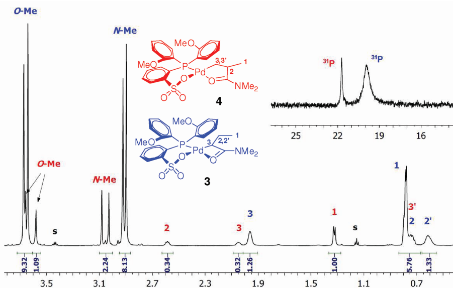
Figure 4. Aliphatic region of ^1\text{H} NMR spectra of dimethyl acrylamide insertion products 3,4 (formed in a 4:1 ratio) in \text{CD}_2\text{Cl}_2 at 25^\circ\text{C} . S: Residual \text{Et}_2\text{O} resonances. Inset: Close up of ^{31}\text{P} NMR spectra of 3,4 under identical conditions.
