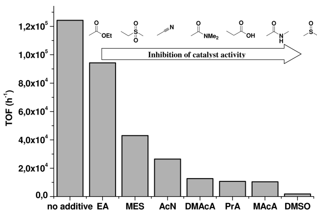
Figure 1. Inhibition of ethylene polymerization by saturated compounds with various polar groups (reaction conditions: 2.5 \mu mol 1-DMSO, 10 bar, 80 °C, 30 min, total volume of toluene and polar compound 50 mL, 0.05 M of additive).
