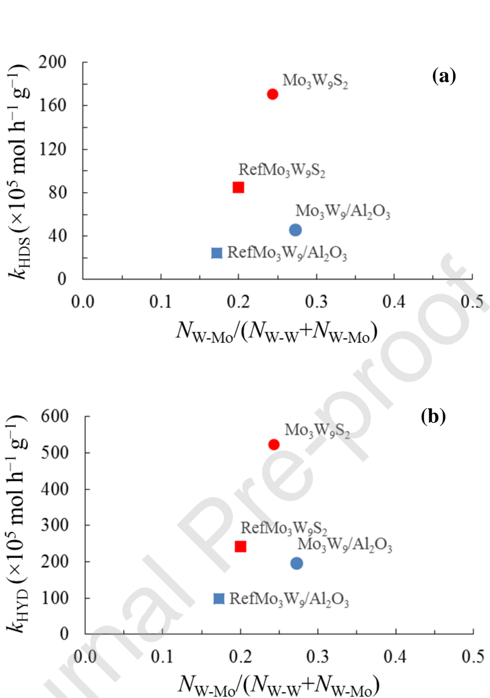
Fig. 10. Activity in DBT HDS (a) and naphthalene HYD (b) over unsupported \text{Mo}_n\text{W}_{12-n}\text{S}_2 and supported \text{Mo}_n\text{W}_{12-n}/\text{Al}_2\text{O}_3 [9] catalysts depending on the W-Mo coordination.
