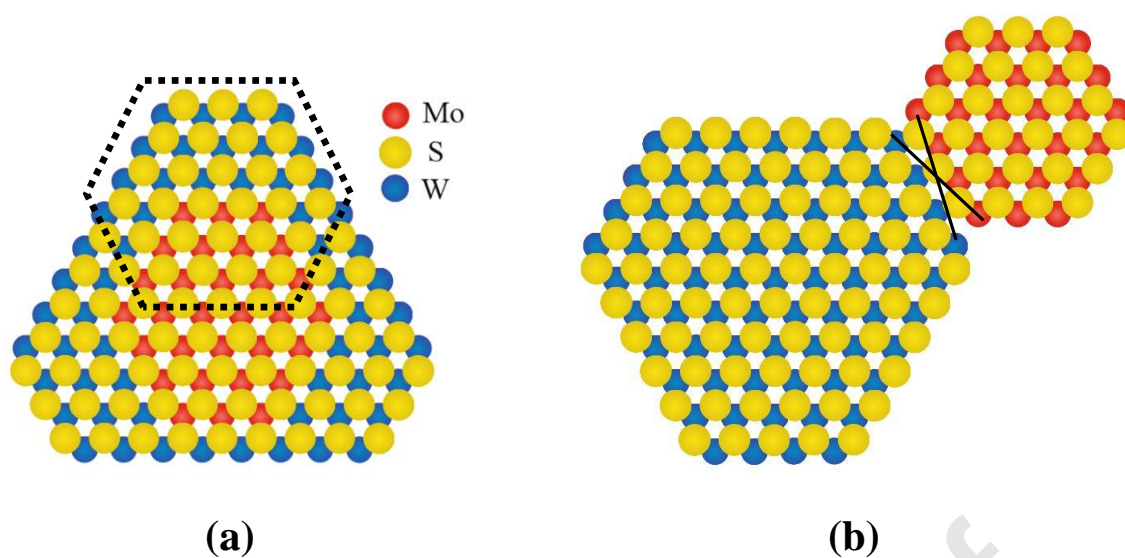
Fig. 9. The possible simplified models of mixed \text{MoWS}_2 active particles in unsupported \text{Mo}_3\text{W}_9\text{S}_2 (a) and \text{RefMo}_3\text{W}_9\text{S}_2 (b) catalysts.
