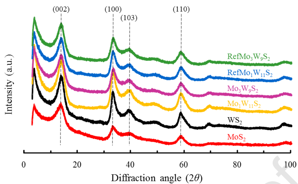
Fig. 3. XRD patterns of unsupported Mo n W 12-n S 2 catalysts.
