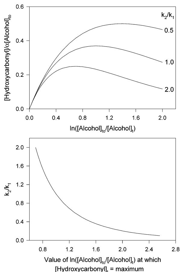
Figure 1. Top: calculated plots of eq II for values of k_2/k_1 = 0.5, 1.0 , and 2.0 . Bottom: plots of values of \ln([\text{alcohol}]_0/[\text{alcohol}]_t) at which [\text{hydroxycarbonyl}]_t is a maximum against the rate constant ratio k_2/k_1 .
