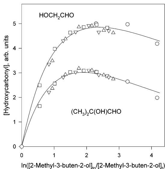
Figure 5. Plots of eq II for the formation of (CH 3 ) 2 C(OH)CHO and HOCH 2 CHO from the OH radical-initiated reaction of 2-methyl-3-buten-2-ol, together with the nonlinear least-squares fits of the data to eq II. The different symbols denote different experiments, and the hydroxycarbonyl concentrations are in arbitrary units based on the GC peak areas.
