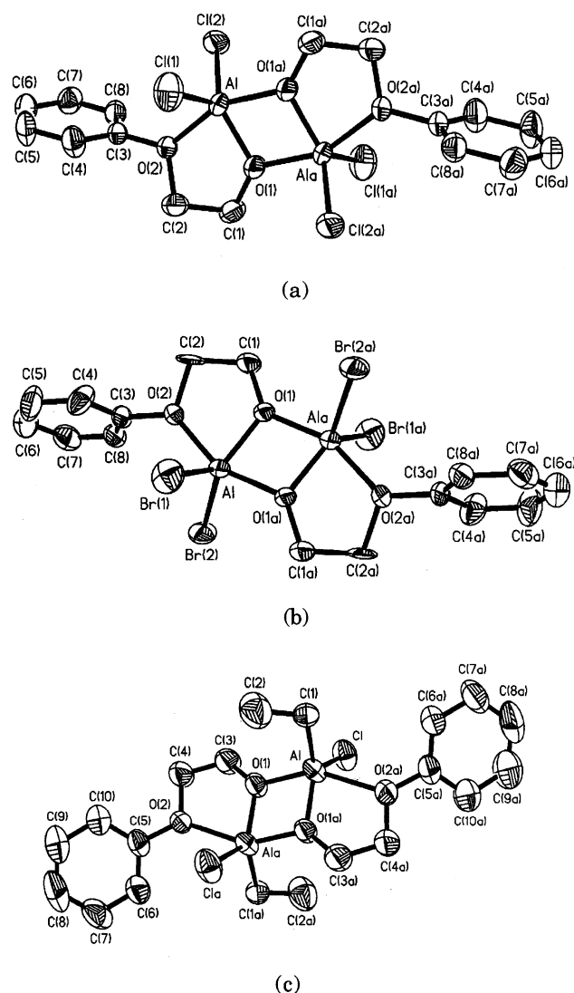
Fig. 1. Molecular structures of (a) [(\mu\text{-OCH}_2\text{CH}_2\text{Oph})\text{AlCl}_2]_2 ( 1 ) (b) [(\mu\text{-OCH}_2\text{CH}_2\text{Oph})\text{AlBr}_2]_2 ( 2 ) and (c) [(\mu\text{-O}(\text{CH}_2)_2\text{Oph})\text{Al}(\text{Et})_{0.75}(\text{Cl})_{1.25}]_2 ( 4 ).
