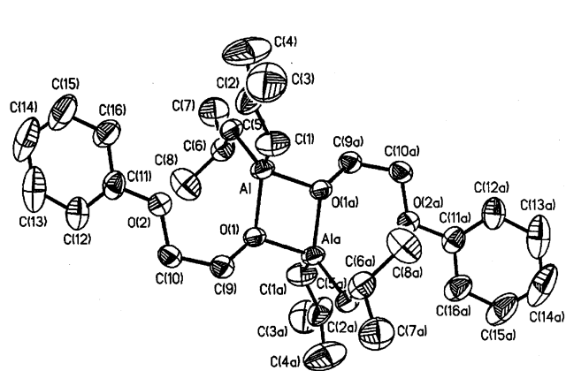
Fig. 2. Molecular structure of (\mu\text{-O}(\text{CH}_2)_2\text{Oph})\text{Al}(\text{Bu}^i)_2]_2 ( 3 ).
