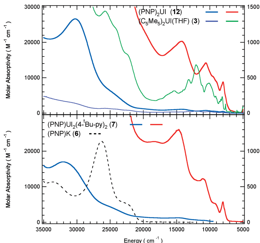
Figure 7. UV–visible–near IR electronic absorption spectral data for toluene solutions of (C_5Me_5)_2UI(THF) ( 3 ), (PNP)K ( 6 ), (PNP)UI_2(4\text{-}t\text{-Bu-py})_2 ( 7 ), and (PNP)_2UI ( 12 ). The left ordinate scale pertains to the UV–visible region (blue, purple, and black spectra) and the right ordinate scale to the near-IR region (red and green spectra).
