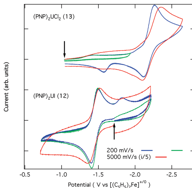
Figure 6. Cyclic voltammograms for (PNP) 2 UI ( 12 ) and (PNP) 2 UCl 2 ( 13 ) in ~0.1 M [Bu 4 N][B(1,3-(CF 3 ) 2 -C 6 H 3 ) 4 ]/THF solution at a Pt working electrode. The vertical arrows indicate the rest potentials of each solution.
