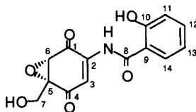
Figure 1. epoxyquinomicin B ( 1 )
