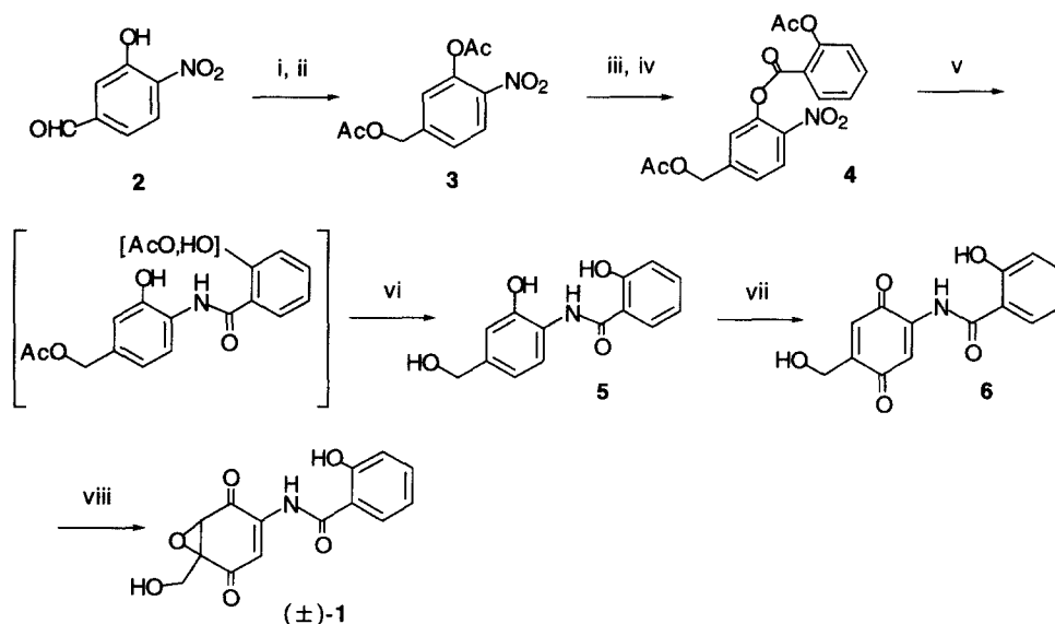
Scheme 1. Reagents and conditions: i, \text{NaBH}_4 , 5% \text{NaHCO}_3 , 0 °C, 30 min; ii, \text{Ac}_2\text{O} , pyridine, room temp., 30 min; iii, \text{KHCO}_3 (1.5 equiv.), MeOH, room temp., overnight; iv, acetylsalicyloyl chloride, 0 °C, 30 min (50% from 2 ); v, \text{H}_2 (1 bar), Raney Ni, AcOEt, AcOH, room temp., 8 h; vi, 1N NaOH, room temp., overnight (64%, 2 steps); vii, Fremy's salt, AcOEt, water, room temp., overnight (82%); viii, \text{H}_2\text{O}_2 , 5% \text{NaHCO}_3 , MeOH, room temp., 2 h, 85%
