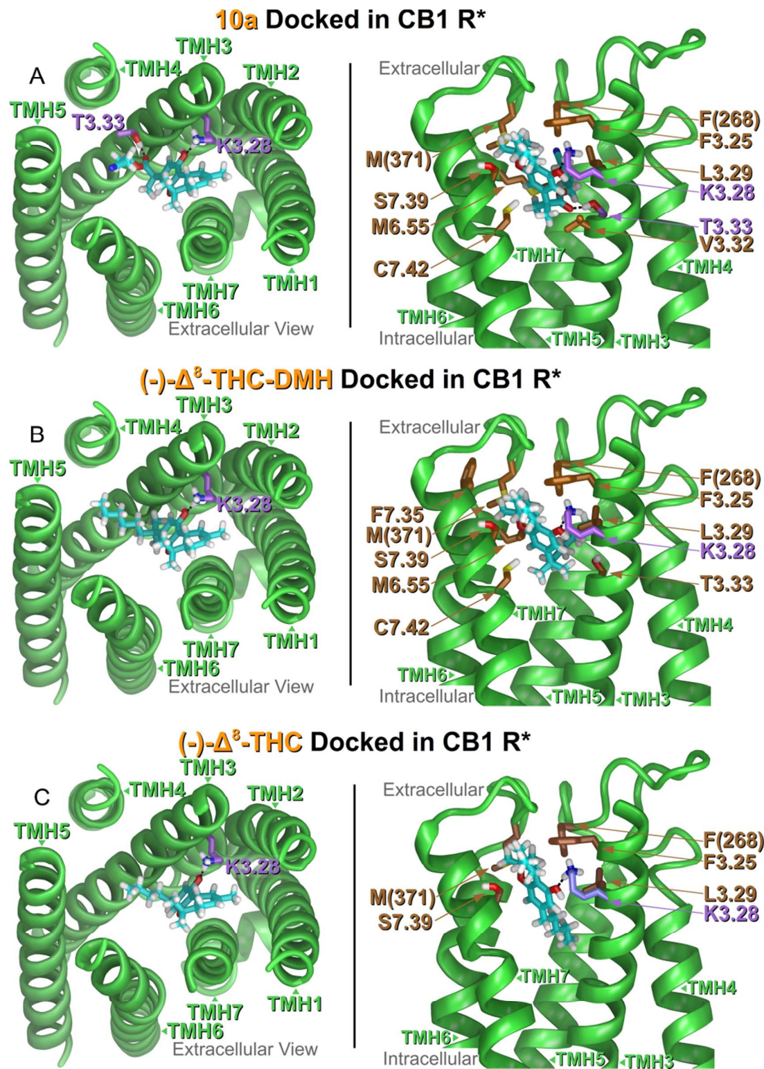
Figure 4A-C. Left panel A-C: Extracellular viewpoint of each ligand/receptor complex. Termini and loops are not shown in this panel. Ligand carbons are colored cyan and hydrophilic interactions
