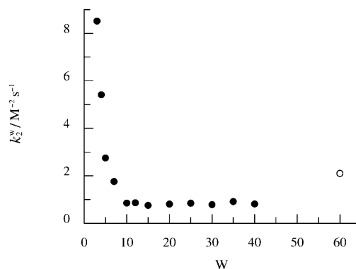
Figure 14. Influence of W on k_2^w for the aminolysis of NPA by sarcosine in AOT/isooctane/water microemulsions at 25 °C (●); [\text{SAR}] = 5.00 \times 10^{-2} \text{ M} referred to the volume of the aqueous microdroplet. Bimolecular rate constant obtained in bulk water (○).
