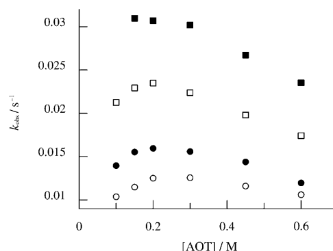
Figure 1. Influence of the microemulsion composition on k_{obs} for the aminolysis of NPA by n -decylamine. [DEC] = 2.50 \times 10^{-2} M referred to the total volume of the system; T = 25^\circ C ; \circ : W = 3 , \bullet : W = 7 , \square : W = 20 , and \blacksquare : W = 35 .
