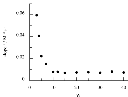
Figure 12. Influence of W on 1/\text{slope} for the aminolysis of NPA by sarcosine in AOT/isooctane/water microemulsions at 25^\circ\text{C} ; [SAR]=5.00 \times 10^{-2} \text{ M} referred to the aqueous phase of the system.
