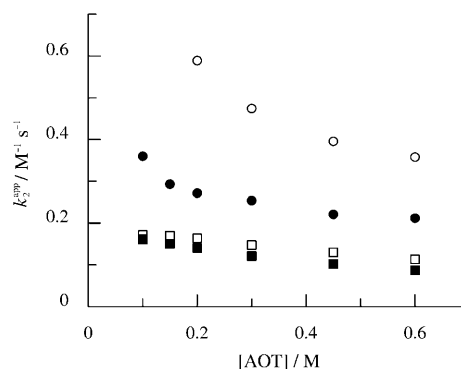
Figure 3. Influence of the microemulsion composition on k_2^{\text{app}} for the aminolysis of NPA by SAR [\text{SAR}] = 5.00 \times 10^{-2} \text{ M} referred to the aqueous phase of the system; T = 25^\circ\text{C} ; \circ : W = 4 , \bullet : W = 7 , \square : W = 15 , and \blacksquare : W = 30 .
