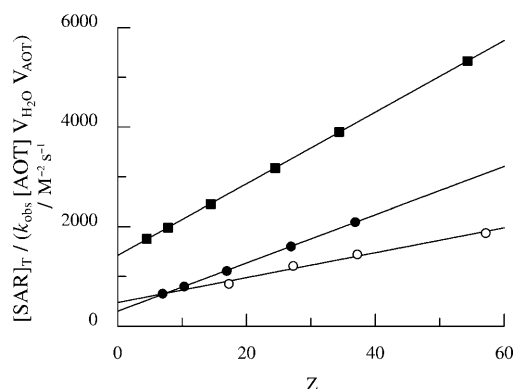
Figure 11. Fit of Equation (15) for the aminolysis of the NPA by SAR; [SAR]=5.00 \times 10^{-2} \text{ M} referred to the aqueous phase of the system; T=25^\circ\text{C} ; \circ : W=4 , \bullet : W=7 , and \blacksquare : W=30 .
