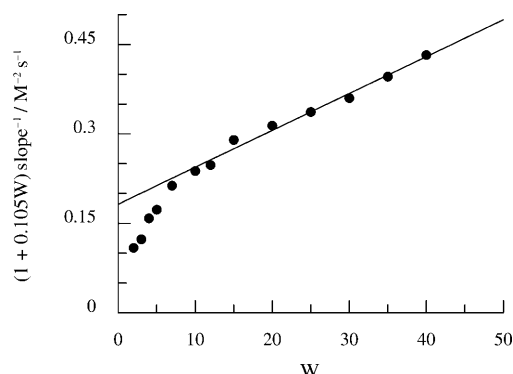
Figure 10. Influence of W on (1+0.105W)/\text{slope} [Eq. (17)] for the aminolysis of NPA by piperazine in AOT/isooctane/water microemulsions at 25°C; [\text{PIP}]=0.10\text{ M} , referred to the aqueous phase of the system. The line represents the fit of Equation (17) to the experimental results; for the fit only the values obtained for W > 10 have been considered.
