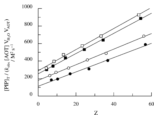
Figure 8. Fit of Equation (15) for the aminolysis of the NPA by PIP. [\text{PIP}] = 0.10\text{M} referred to the aqueous phase of the system; T = 25^\circ\text{C} ; \bullet : W = 7 , \circ : W = 15 , \blacksquare : W = 30 , and \square : W = 40 .
