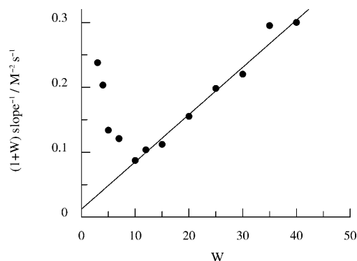
Figure 13. Influence of W on (1+W)/\text{slope} [Eq. (19)] for the aminolysis of NPA by sarcosine in AOT/isooctane/water microemulsions at 25 °C; [\text{SAR}] = 5.00 \times 10^{-2} \text{ M} , referred to the aqueous phase of the system; the line represents the fit of Equation (19) to the experimental results. For the fit only the values obtained for W > 10 have been considered.
