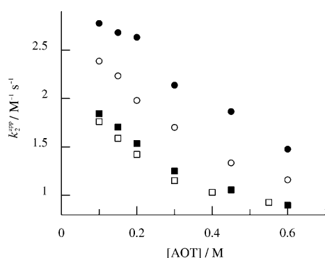
Figure 2. Influence of the microemulsion composition on k_2^{\text{app}} in the aminolysis of NPA by PIP. [\text{PIP}]_{\text{T}} = 0.10 \text{ M} referred to the aqueous phase of the system; T = 25^\circ\text{C} ; \bullet : W = 7 , \circ : W = 15 , \blacksquare : W = 30 , and \square : W = 40 .
