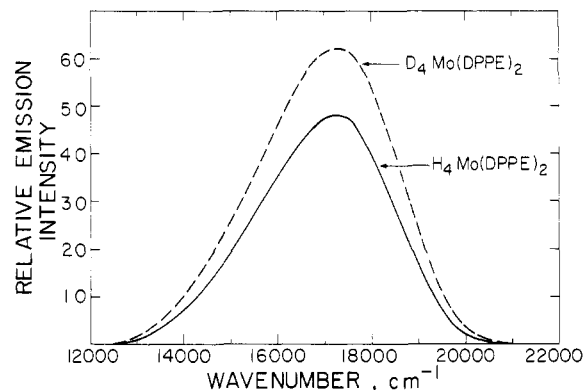
Figure 1. Corrected emission spectral distribution for H_4Mo(DPPE)_2 (—) and D_4Mo(DPPE)_2 (---) in 2-methyltetrahydrofuran at 77 K. The excitation wavelength is 390 nm. See Table I for quantum yields.
