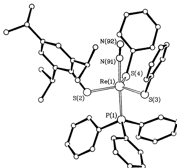
Fig. 3 An ORTEP representation of one of the two virtually identical molecules of [\text{Re}(\text{SC}_6\text{H}_2\text{Pr}^i_{3-2,4,6})_3(\text{N}_2)(\text{PPh}_3)] 4 with some isopropyl groups omitted for clarity and with a partial atom labelling scheme
