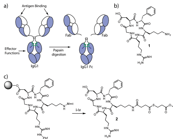
Figure 1. Antibody fragments and RGD peptides. (a) Antibody fragments obtained upon protease digestion. (b) Cyclic-RGDfK \alpha_v\beta_3 integrin antagonist 1 . (c) Solid-phase synthesis of cyclic RGDfK thioester derivative 2 : (i) 1% TFA in \text{CH}_2\text{Cl}_2 ; (ii) succinic anhydride and N -methylmorpholine; (iii) methyl 3-mercaptopropionate, DIC, HOBT, DMAP; (iv) TFA with TIS.
