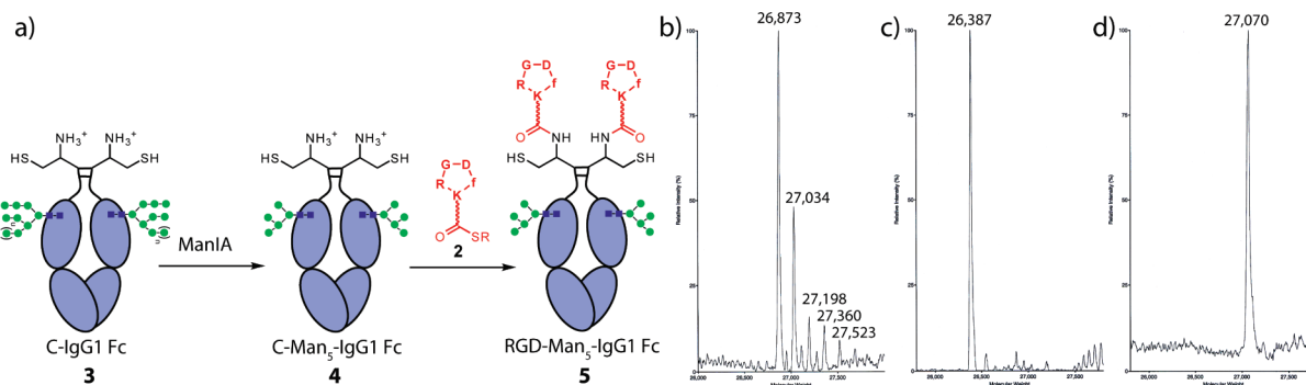
Figure 2. Synthesis of RGD-Man 5 -IgG1 Fc. (a) Conversion of C-IgG1 Fc ( 3 ) to RGD-Man 5 -IgG1 Fc ( 5 ) by ManIA digestion and NCL with thioester 2 . (b) ESI-MS of heterogeneously glycosylated C-IgG1 Fc ( 3 ). Calcd molecular weights for glycoforms containing 8–12 mannose residues: 26 872, 27 035, 27 198, 27 361, and 27 524, respectively. (c) ESI-MS of 4 : calcd, 26 386; obsd, 26 387. (d) ESI-MS of 5 : calcd, 27 071; obsd, 27 070.
