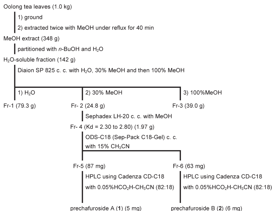
Chart 1. Isolation of Prechafuroside A (1) and Prechafuroside B (2) from Oolong Tea Leaves from Shizu 7132, Camellia sinensis (L.) O. Kuntze
