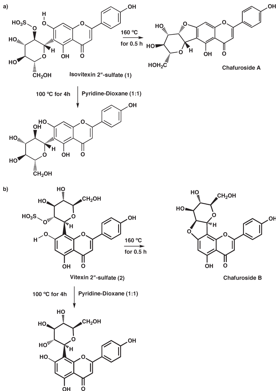
Figure 4. Preparation of (a) chafuroside A and isovitexin from isovitexin 2''-sulfate (1) and (b) chafuroside B and vitekin from vitekin 2''-sulfate (2).
