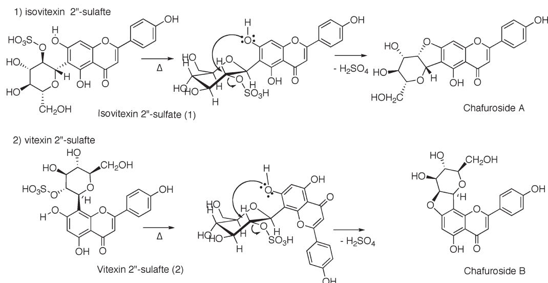
Figure 6. Proposed formation mechanisms of etheric bond in isovitexin 2''-sulfate (1) and vitexin 2''-sulfate (2).
