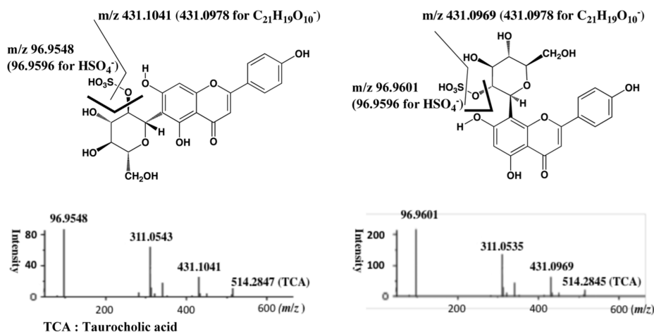
Figure 5. Negative MS/MS spectra of (A, left) isovitexin 2''-sulfate (1) and (B, right) vitexin 2''-sulfate (2).
