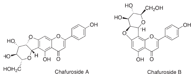
Figure 1. Structures of chafuroside A and B from oolong tea.
