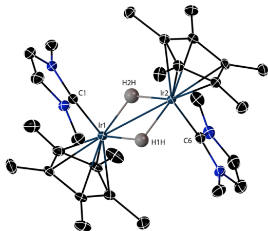
Figure 1. X-ray crystal structure of complex 5 . Ellipsoids are at the 50% probability level. Hydrogen atoms and triflate counterions were omitted for clarity. Selected bond lengths (Å) Ir1-Ir2, 2.7118(6); Ir1-C1, 2.0266(18); Ir2-C6, 2.0238(18).
