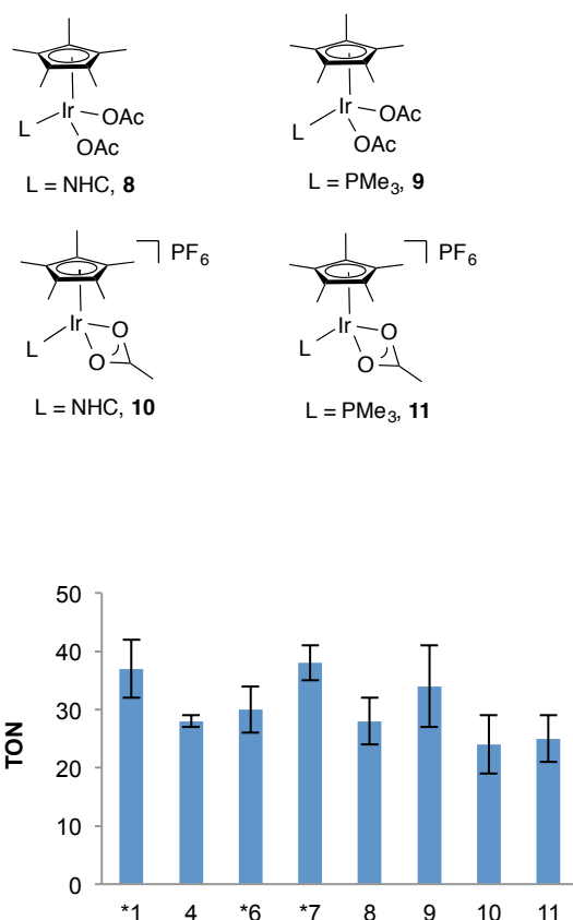
Figure 2. Catalytic H/D exchange reactions with complexes 1 , 4 , 6 , 7 , 8 , 9 , 10 and 11 in acetic acid- d 4 . Conditions: Reactions were run for 24 h with 25 equivalents of deuterium source to C 6 H 6 . The reported turnover numbers are the average of at least three trials and error is reported as the standard deviation of the mean. * 2 equivalents of AgOTf were added to the complex.
