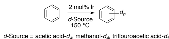
Scheme 1. Ir-catalyzed H/D exchange
