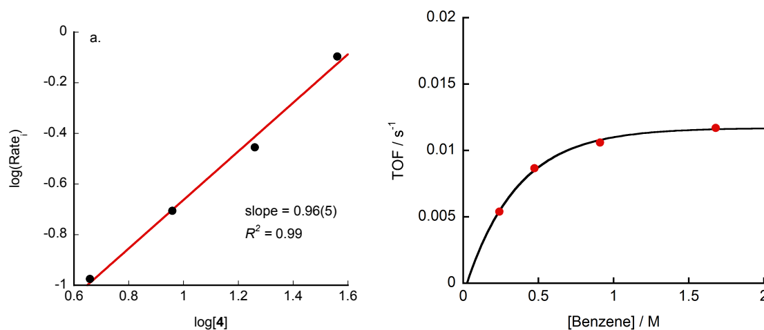
Figure 3. a) Plot of initial rate of deuterium incorporation versus [4] in methanol- d 4 b) Plot of turnover frequency versus [benzene] in methanol- d 4 . Conditions: (a) Ir catalyst (0.0024, 0.0028, 0.0095, 0.019 mmol), benzene (0.475 mmol), methanol- d 4 (11.9 mmol) at 150 °C for 0.5 h. (b) Ir catalyst (0.0095 mmol), benzene (0.238, 0.475, 0.950, 1.68 mmol), methanol- d 4 (11.9 mmol) at 150 °C for 0.5 h. Data are fit with nonlinear least-squares fitting to an equation describing saturation in [benzene]: k_{\text{obs}} = k_2[\text{benzene}]/k' + [\text{benzene}] where k' = (k_{-1}[\text{H}^+] + k_2)/k_1 . Turnover frequencies were determined by GC/MS.
