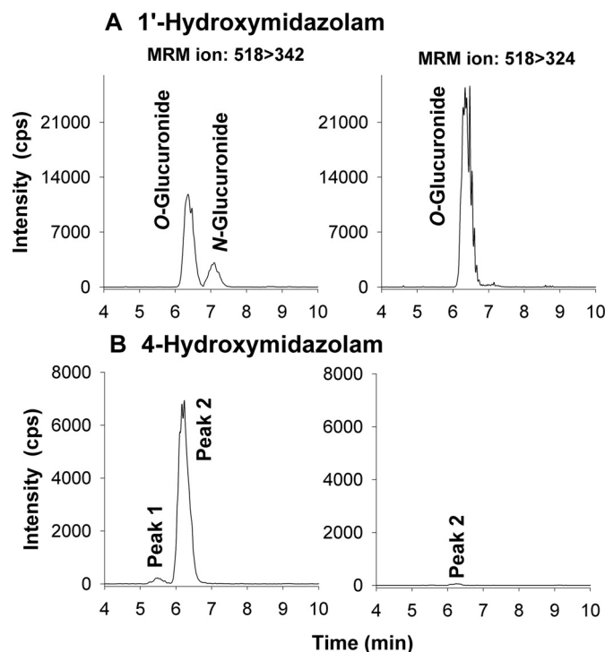
FIG. 2. Multiple-reaction-monitoring (MRM) chromatogram of glucuronide metabolites obtained by LC-MS/MS using HLM incubates of 1'- (A) and 4-hydroxymidazolam (B) in the presence of UDPGA.
