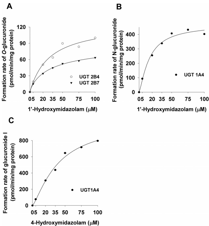
FIG. 7. Representative Michaelis-Menten plots for glucuronide conjugate formation from 1'-hydroxymidazolam (A and B) and 4-hydroxymidazolam (C) by recombinant UGT isoforms 1A4, 2B4, and 2B7. The recombinant UGT isoforms (0.25 mg/ml) were incubated with 0 to 100 \mu M 1'- or 4-hydroxymidazolam at 37°C for 60 min in the presence of UDPGA (5 mM). Each data point represents the average of triplicate incubations.
