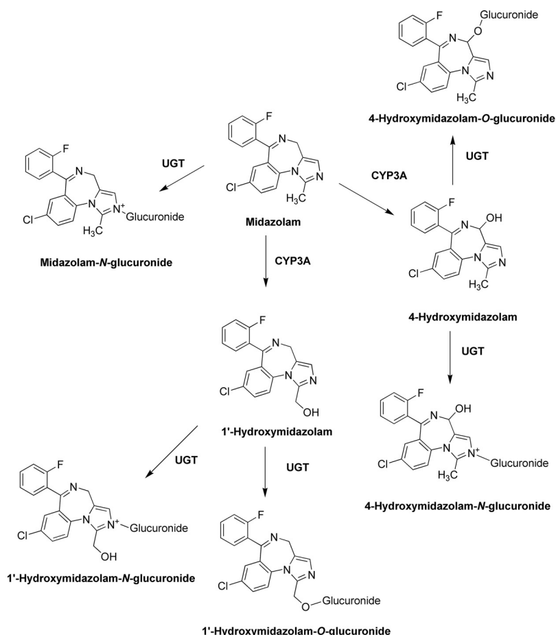
FIG. 1. Proposed pathway of midazolam metabolism in HLMs.
