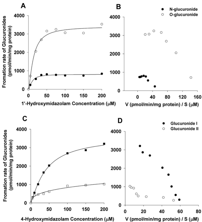
FIG. 6. Representative Michaelis-Menten (left panels) and Eadie-Hofstee (right panels) plots of the glucuronide conjugation of 1'- (A and B) and 4-hydroxymidazolam (C and D). HLMs were incubated with 0 to 200 \mu M 1'-hydroxymidazolam or 4-hydroxymidazolam at 37°C for 60 min in the presence of UDPGA (5 mM). The data points represent the averages obtained from three different HLMs.
