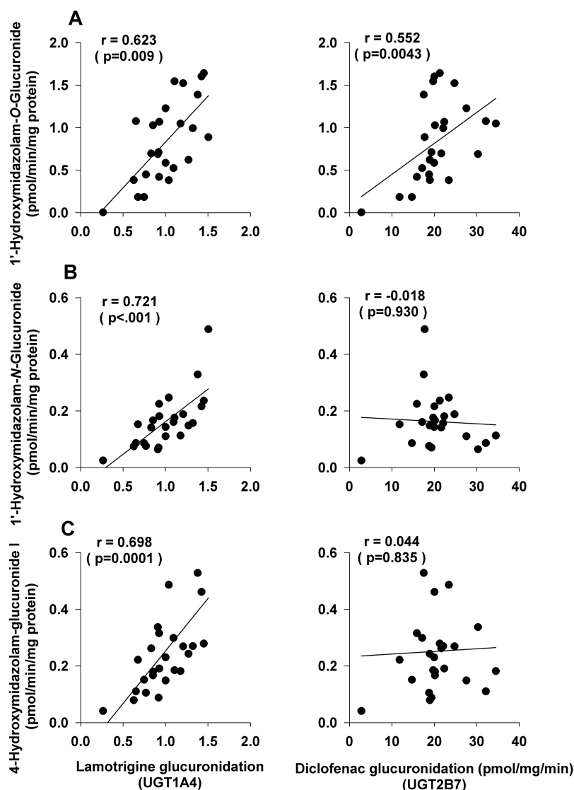
FIG. 5. Simple regression analysis of lamotrigine or diclofenac glucuronidation and the rates of 1'-hydroxymidazolam O -glucuronidation (A) and N -glucuronidation (B) and 4-hydroxymidazolam glucuronide I formation (C) in 25 different HLMs.
