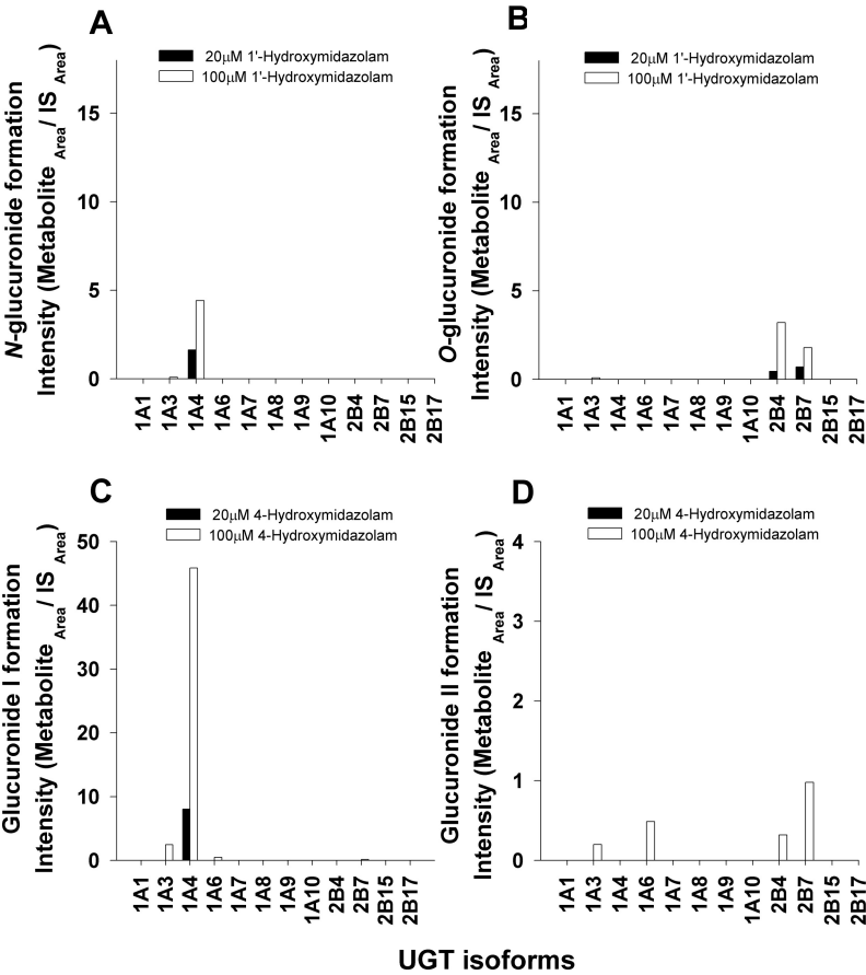
FIG. 3. Representative plots of the formation of 1'-hydroxymidazolam N -glucuronide (A) and O -glucuronide (B) from 1'-hydroxymidazolam, from 4-hydroxymidazolam glucuronides I (C) and II (D) and from 4-hydroxymidazolam by recombinant human UGT isoforms. IS, internal standard.
