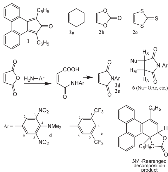
Figure 1. Structures and atom numbering for key reagents, precursors and possible side-products.
