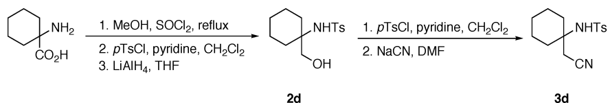
Scheme 2 Preparation of nitrile 3d .
