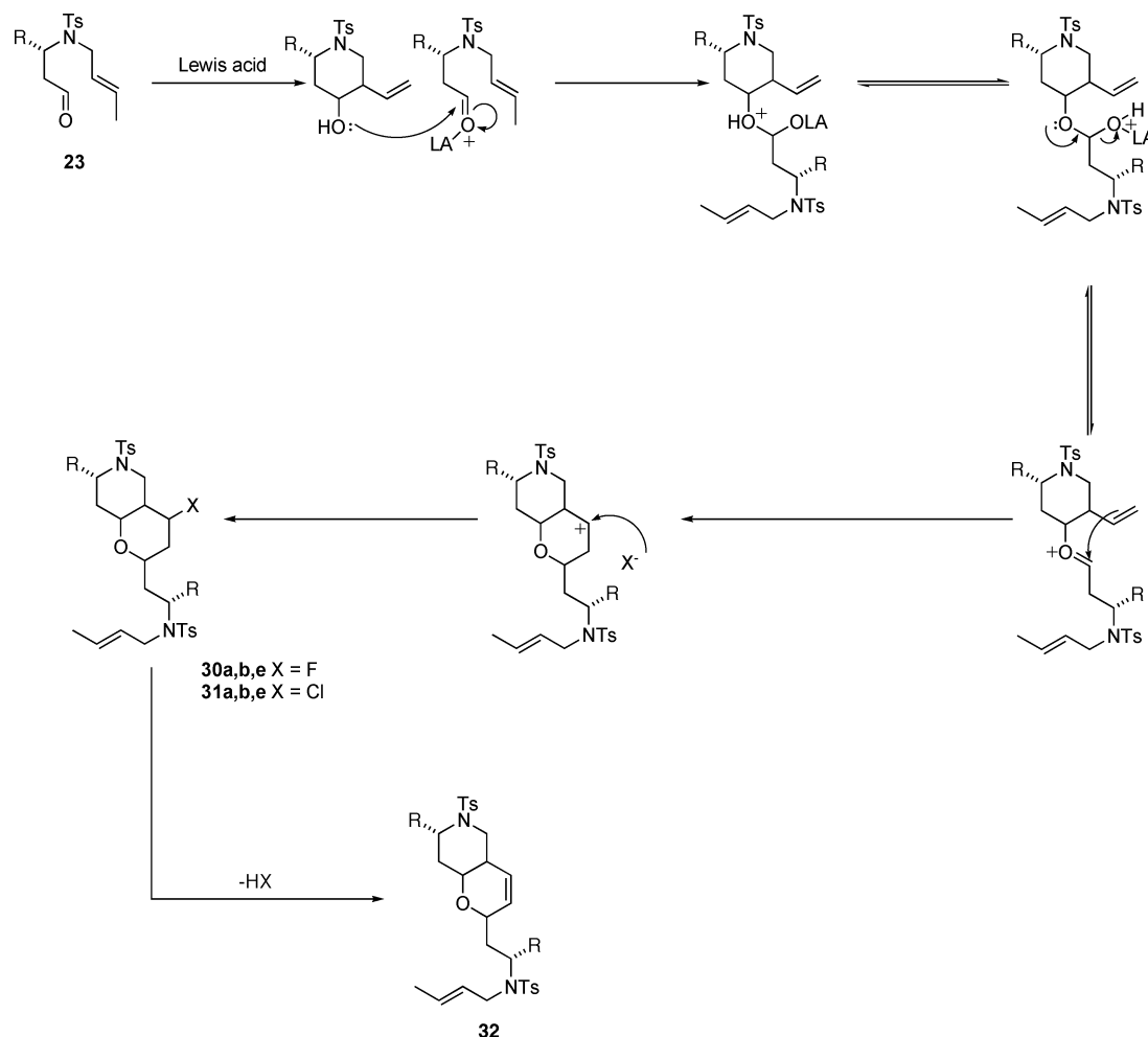
Scheme 13 Proposed route to dimerisation products.
