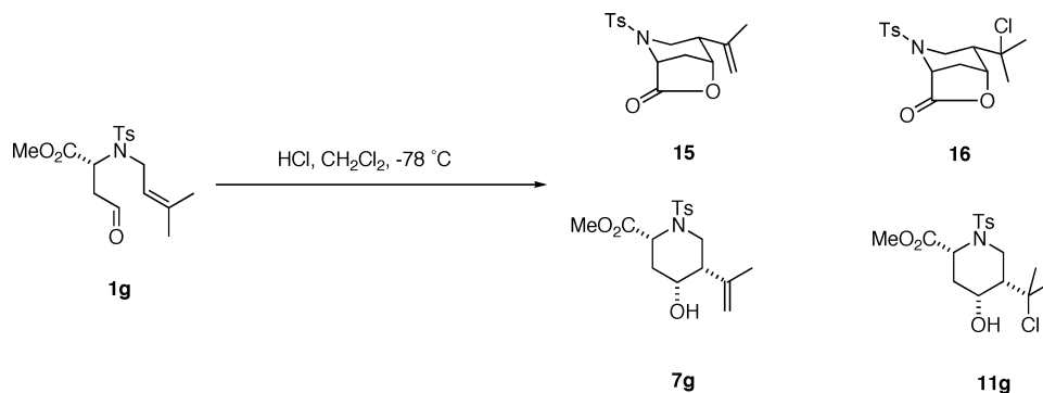
Scheme 9 Brønsted acid-catalysed cyclisation of 1g .
