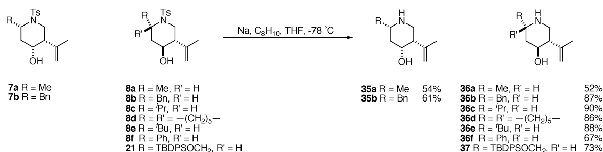
Scheme 15 Removal of the p -toluenesulfonyl protecting group.
