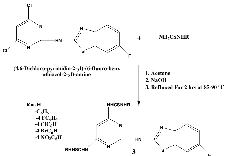
Scheme 1. Synthetic procedure for preparation of 2-(6'-fluorobenzothiazol-2'-ylamino)-4,6-(disubstituted thiouriedo)-1,3-pyrimidine derivatives
