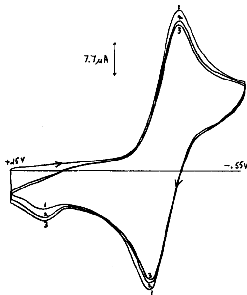
Figure 1. Multicycle voltammogram of trans -[Mo(CO) 2 dpe 2 ] + BF 4 - at a vitreous carbon electrode in CH 2 Cl 2 -MeOH-0.1 N Et 4 NBF 4 at \nu = 0.09 V sec -1 .
