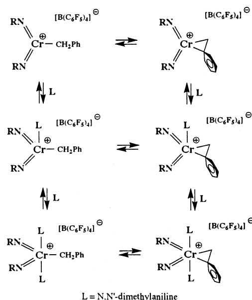
Scheme 2. Possible initiating species arising from the reaction of (\text{RN})_2\text{Cr}(\text{CH}_2\text{Ph})_2 with [\text{PhNMe}_2\text{H}][\text{B}(\text{C}_6\text{F}_5)_4] .
