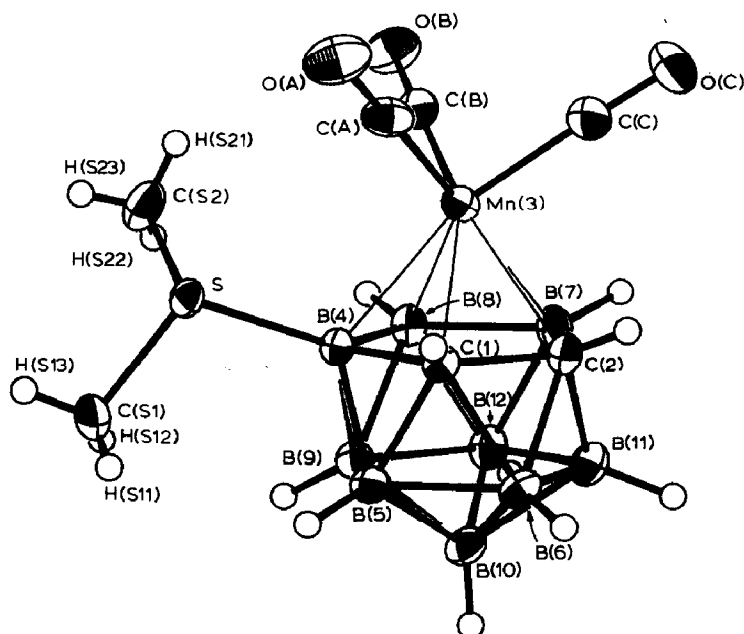
Fig. 1. Perspective view of compound 1. All atoms drawn as 50% probability ellipsoids, except for H atoms which have an artificial radius of 0.1 Å for clarity. Cage H atoms carry the same number as the B or C to which they are bound.
