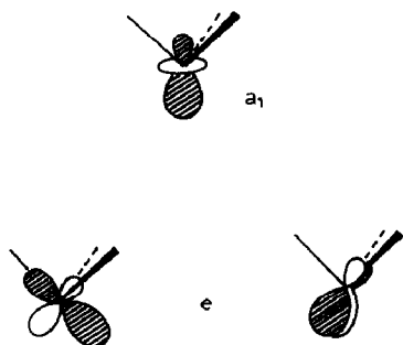
Fig. 5. The e and a_1 acceptor orbitals of \{\text{Mn}(\text{CO})_3\}^+ .
