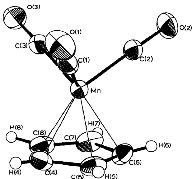
Fig. 3. Perspective view of compound 2. Thermal ellipsoids as for Fig. 1.
