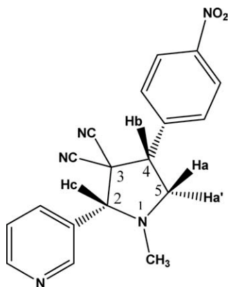
Scheme 2. Structure of derivative 3a .
