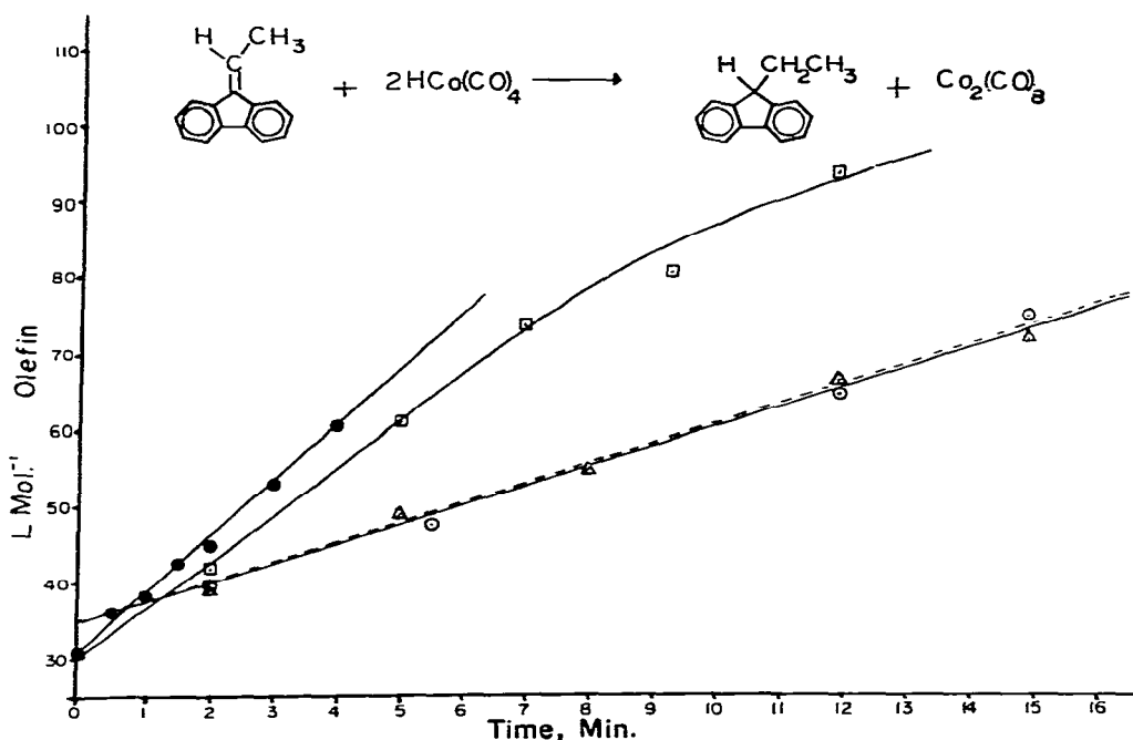
Fig. 1. Second order plot of conversion of 9-ethylidene fluorene (IIb): ● at 0°C under CO; ◻ at -10°C under CO using DCo(CO) 4 ; △ at -10°C under N 2 ; ○ at -10°C under CO.
