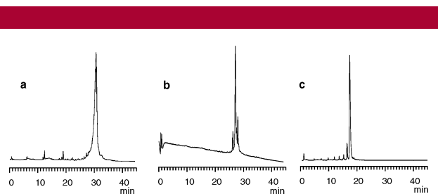
Figure 2. Anion-exchange HPLC profiles of crude mixtures obtained by RNA–DNA chimeric and RNA oligomer syntheses: (a) 2'-OMe-[CCUACAGAGAACUGCGGUU]-TT ( 17 ), (b) 2'-OMe-[GAUACA bz UUGACCU] ( 18 ), and (c) r[CUCUCUCUCU]-T ( 19 ).
