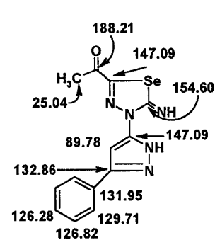
13 C NMR Spectra of 10a
