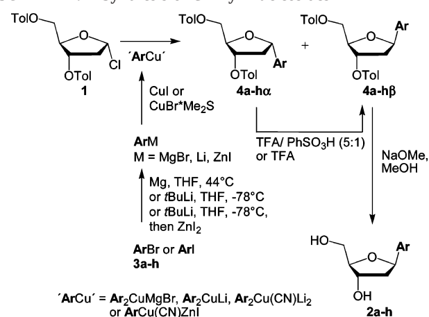
SCHEME 1. Synthesis of C-Aryl-Nucleosides
