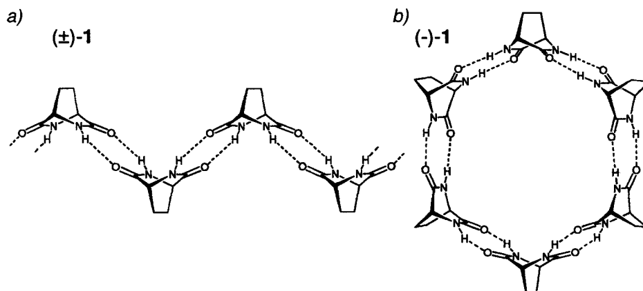
Figure. Possible H-bonding patterns for a) (±)-1 and b) (-)-1
