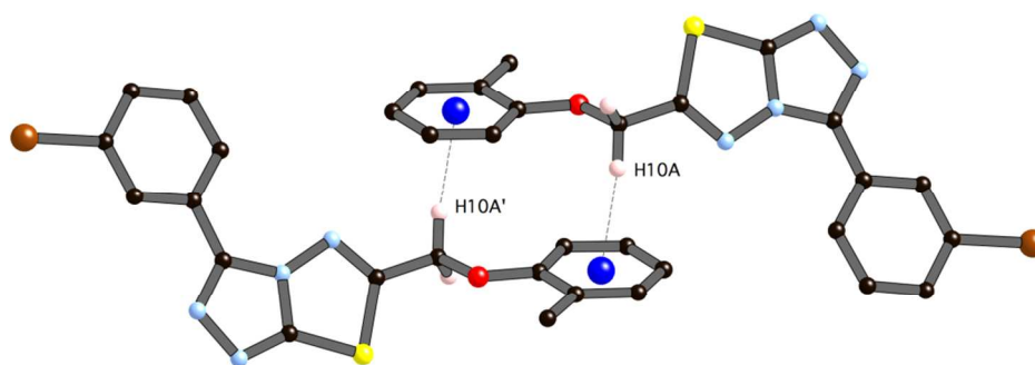
Fig. 5 C-H... \pi interaction between centrosymmetrically related pairs of 4i , symmetry operator (1-x, -y, -z) .
