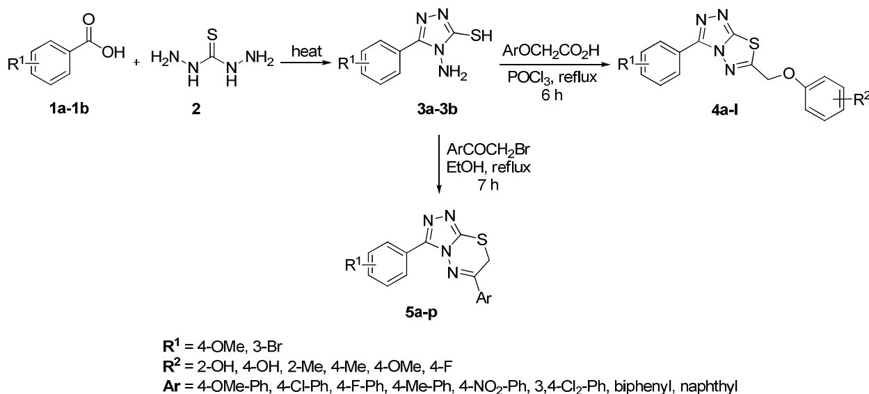
Scheme 1 Synthesis of triazolothiadiazoles ( 4a-l ) and triazolothiadiazines ( 5a-p ).
