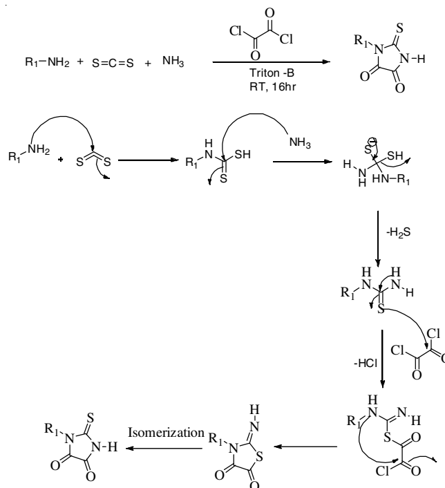
Scheme-I: Synthesis of 2-thioxoimidazolidine-4,5-dione catalyzed by Triton-B
