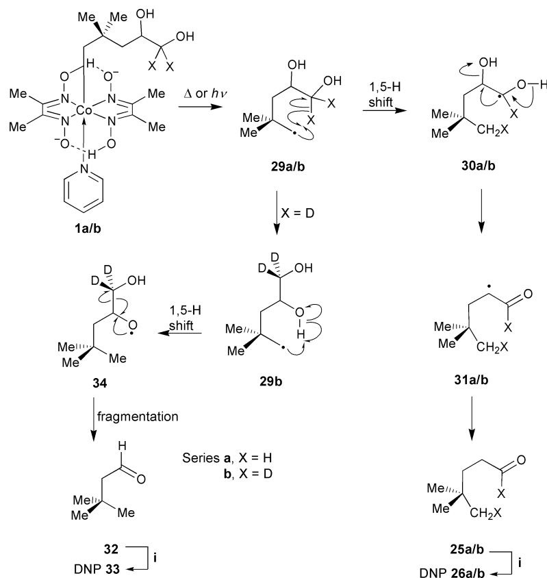
Scheme 3 Thermal and photochemical decomposition of the diol dehydratase model. Reagents and conditions: i 2,4-Dinitrophenylhydrazine, \text{H}_2\text{SO}_4 (aq.), rt.
