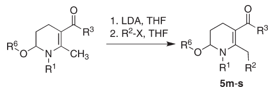
SCHEME 3. Introduction of Substituents at the C 2 -CH 3 Group in 6-Alkoxy-1,4,5,6-tetrahydropyridines
