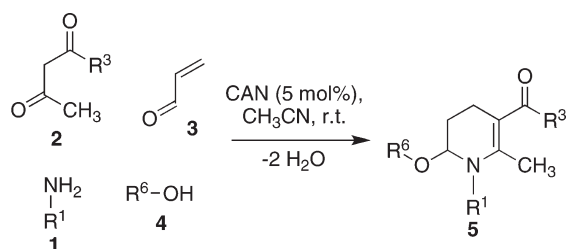
SCHEME 2. Synthesis of Starting 6-Alkoxy-1,4,5,6-tetrahydropyridines
