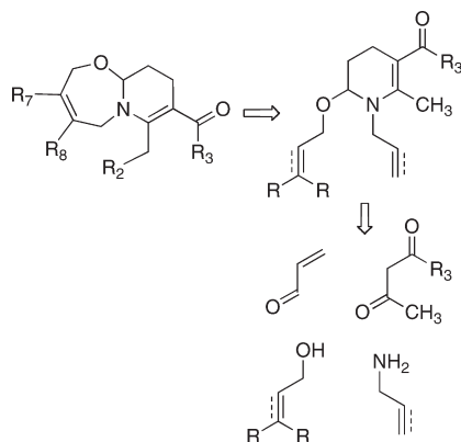
SCHEME 1. Plan for the Synthesis of Pyrido[2,1- b ]-[1,3]oxazepines
