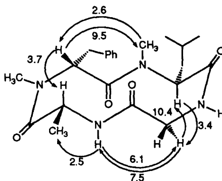
Fig. 13. \text{DNOE} (300 MHz, \text{CDCl}_3 ) Results for 32e
