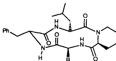
Scheme 1. Four Representatives of Natural Cyclic Tetrapeptides
