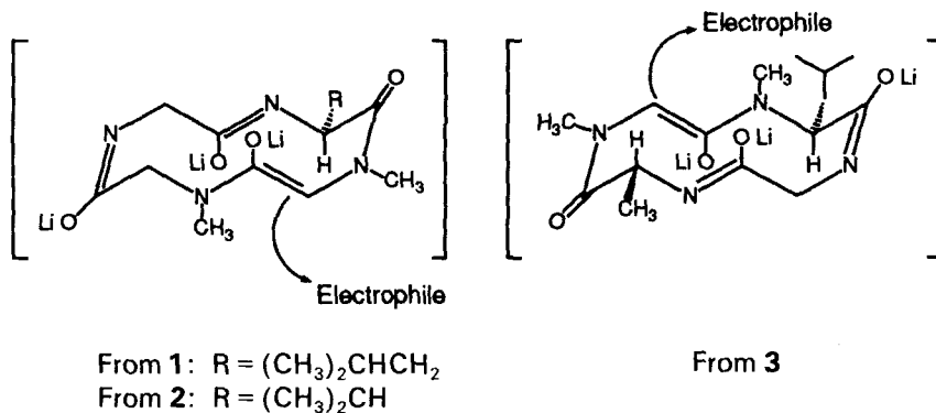
Fig. 5. Proposed structures of the trilitio derivatives of 1 , 2 , and 3 . There are two aza-enolate moieties, one with a (Z)- and one with an (E)-configuration, and a (Z)-enolate in each. The conformations are derived from the major solution conformation of 1 and 2 , and from the only observed solution conformation of 3 .
