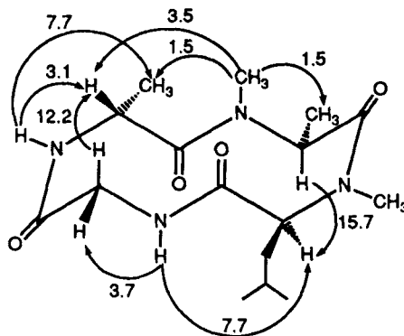
Fig. 14. \text{DNOE} (300 MHz, \text{CDCl}_3 ) Results for 33
