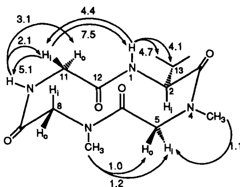
Fig. 7. NOE (300 MHz, (D_6) DMSO) Results for 2
