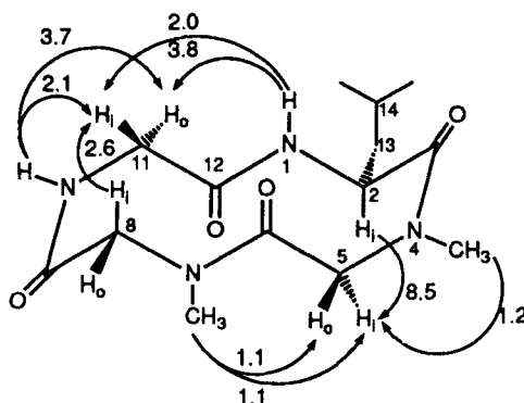
Fig. 6. NOE (300 MHz, (D_6) DMSO) Results for 1 . Enhancements are given in %. For clarity, those enhancements less than 1 %, and of geminal substituents, are not shown.
