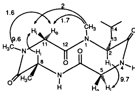
Fig. 8. NOE (300 MHz, \text{CDCl}_3 ) Results for 3
