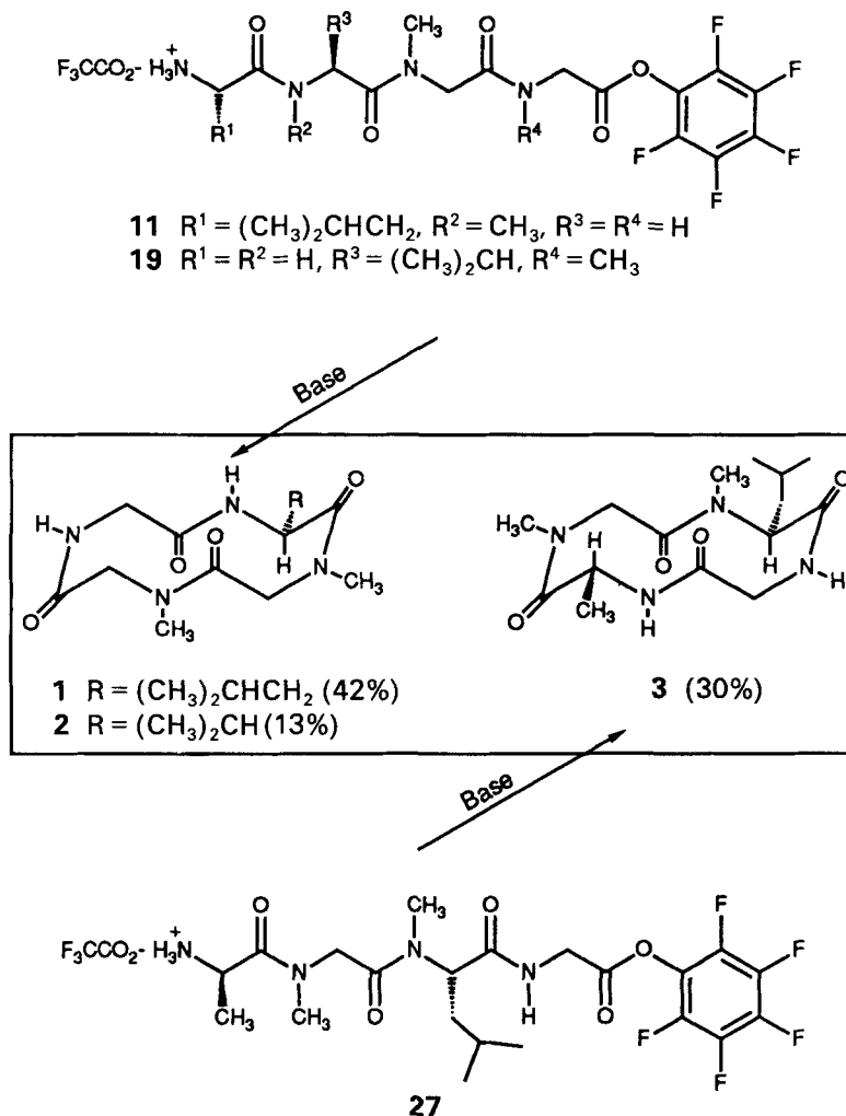
Scheme 3. Cyclization of the Linear Tetrapeptide Pentafluorophenyl Esters 11 , 19 , and 27 to the Cyclic Tetrapeptides 1–3 . High-dilution conditions were employed, with pyridine (20%)/dioxane as solvent, containing 0.8 equiv. of DMAP and 1.5% \text{CF}_3\text{CH}_2\text{OH} .
