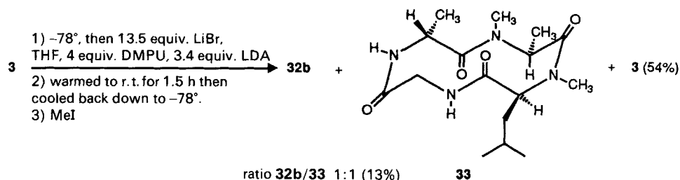
Scheme 5. Alkylation of 3 after Warming the Enolate to Room Temperature. The electrophile was added to the reaction solution at -78^\circ .
