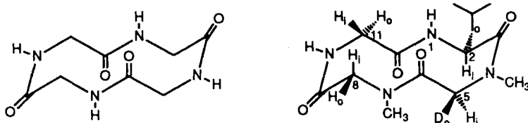
Fig. 1. C_2 -Symmetrical conformation of the unsubstituted backbone of a cyclic tetrapeptide with numbering convention 9) shown for 28a
