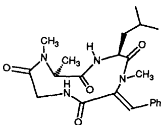
Scheme 1. Four Representatives of Natural Cyclic Tetrapeptides
