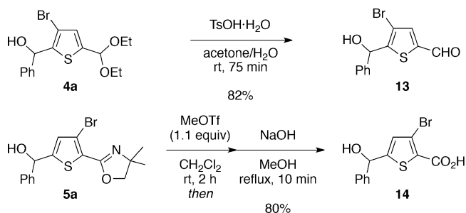
Scheme 3. Conversion of Acetal and Oxazoline Moieties to Formyl and Carboxyl Groups
