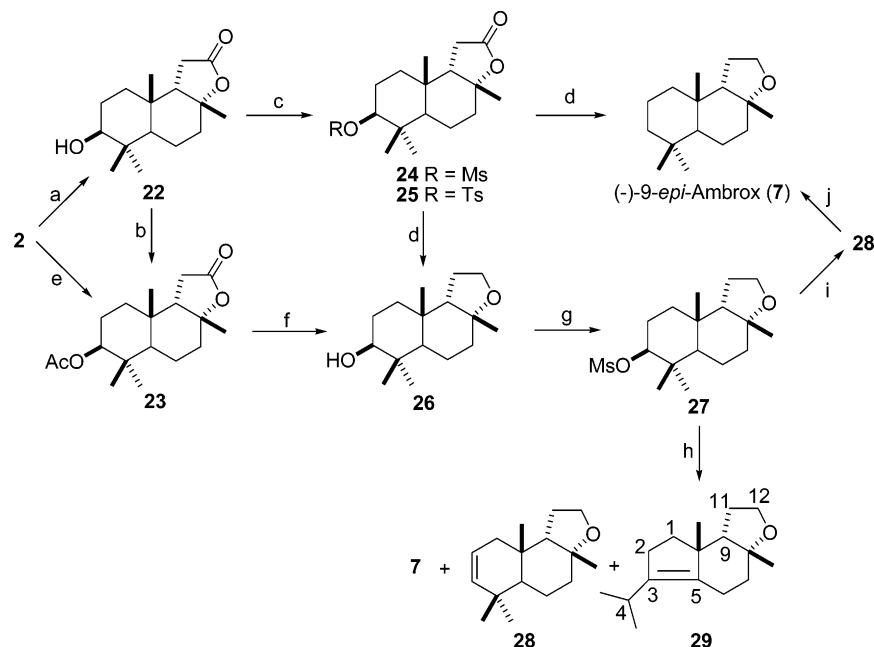
Scheme 6. Synthesis of (–)-9- epi -Ambrox (7) a
