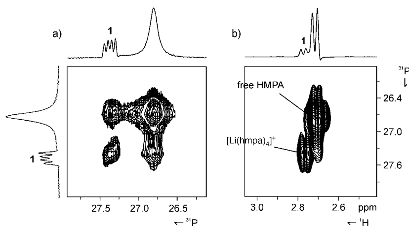
Figure 4. a) 2D ^{31}\text{P} , ^{31}\text{P} EXSY NMR (161.92 MHz) and b) 2D gHMQC (400.13 MHz) of the 60 mm sample LiCl plus HMPA in THF at 155 K. The [\text{Li}(\text{hmpa})_4]^+ ion is indicated as 1 .
