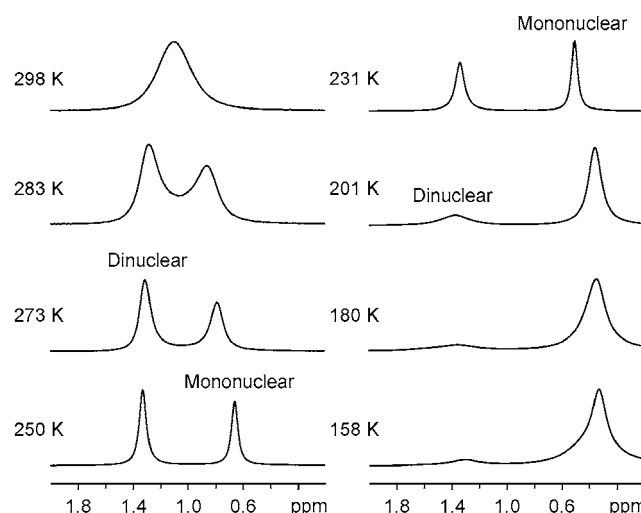
Figure 7. Variable-temperature ^7\text{Li} NMR spectra of a 0.6 M solution of LiHMDS 16 in THF (155.45 MHz).
