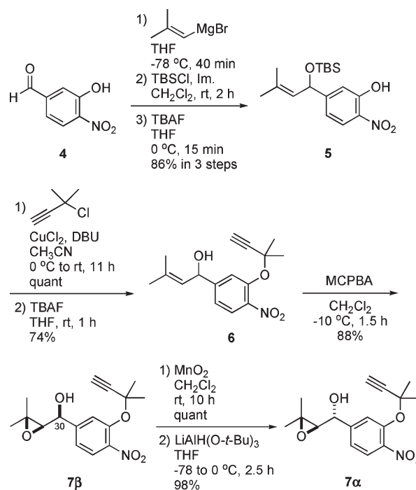
Scheme 1. Synthesis of syn -Epoxyalcohol 7β and anti -Epoxyalcohol 7α
