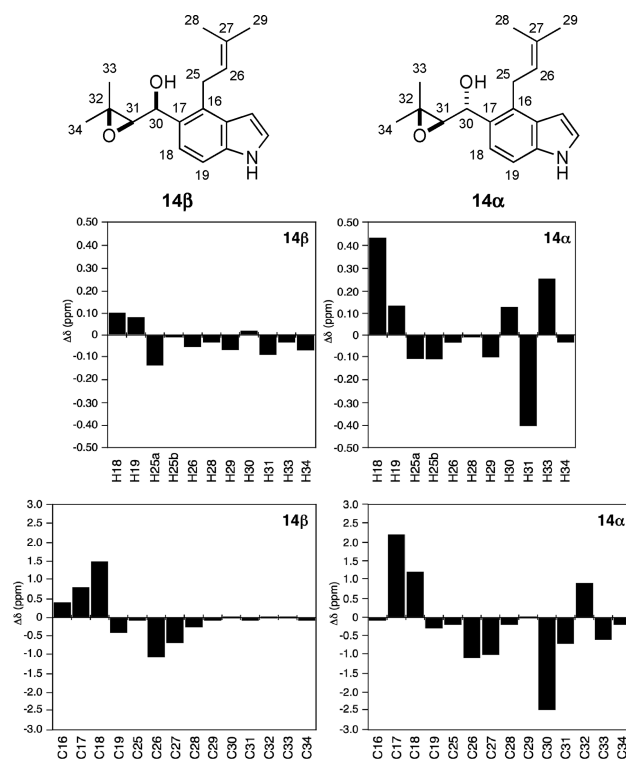
Figure 2. Chemical shift differences ( \Delta\delta ) of 1 H and 13 C NMR spectra for syn - and anti -epoxyindoles 14 . \Delta\delta = \delta (synthetic) – \delta (natural). Bars represent the deviation in ppm between individual chemical shifts observed for 14 and those reported for the spendole ( 1 ) (400 MHz, C 5 D 5 N).
