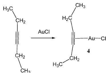
Scheme 1. Synthesis of Au(EtC≡CEt)Cl
