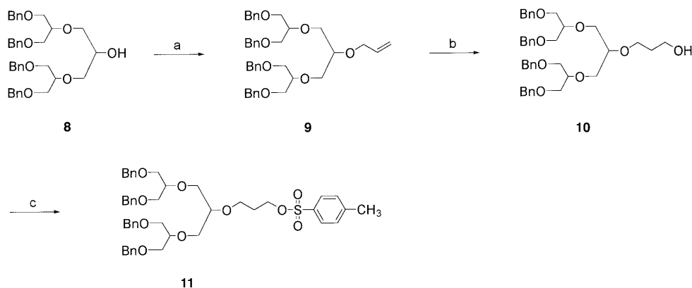
Scheme 2. Synthesis of p -toluene sulfonate derivative of cascade polyol. Reaction condition: (a) allyl bromide, NaH, DMF; (b) (i) (9-borabicyclo[3.3.1]non-2-yl)BH, THF (ii) p -TsCl, pyridine.
