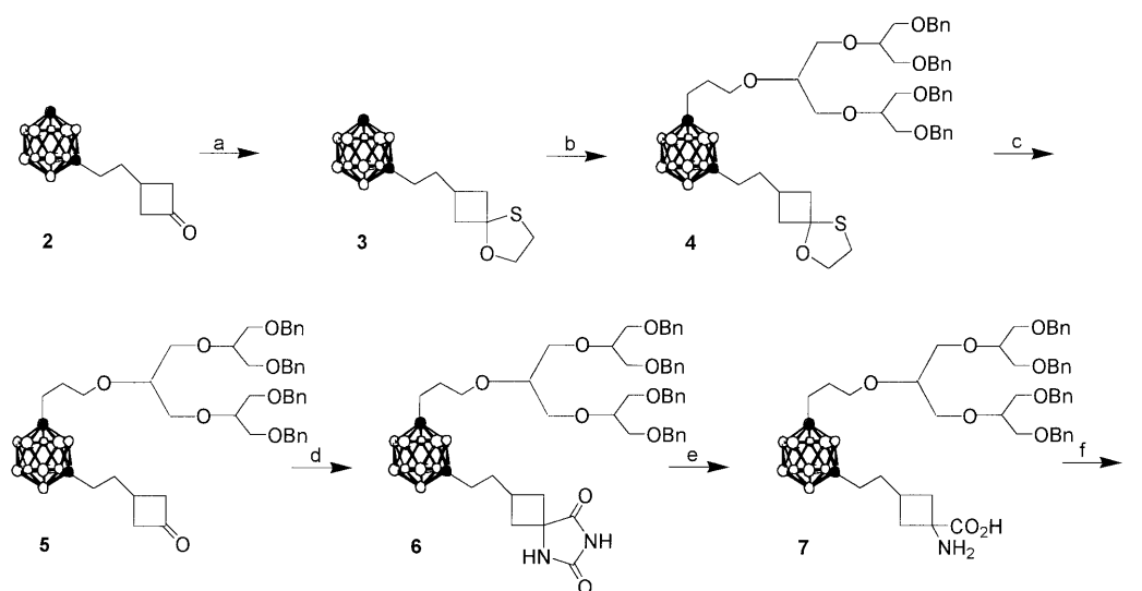
Scheme 1. Synthesis of cascade polyol-containing meta -carbonyl ACBC: Reaction condition: (a) \text{HO}(\text{CH}_2)_2\text{SH} , \text{TsOH} , \text{C}_6\text{H}_6 ; (b) \text{BuLi} , THF, 11 ; (c) \text{HgCl}_2 , 0.1 N \text{NaOH} , THF; (d) \text{KCN} , (\text{NH}_4)_2\text{CO}_3 , aqueous EtOH (50% solution in \text{H}_2\text{O} ); (e) 2 N \text{NaOH} ; (f) \text{H}_2 , Pd-C, MeOH.
