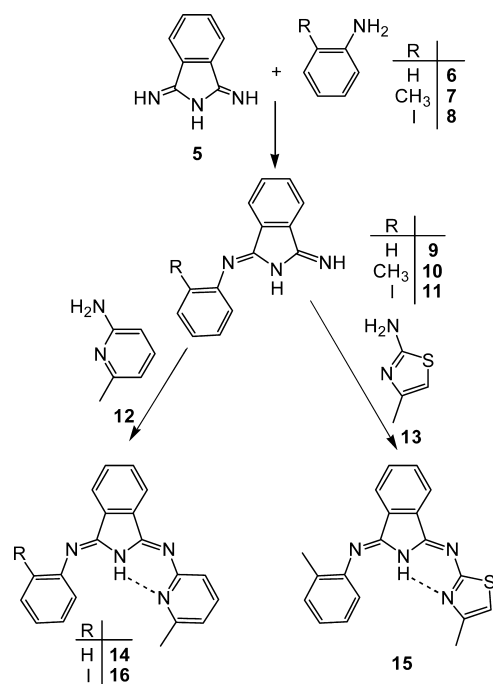
Scheme 2. Two-Step Preparation of Unsymmetric H(bai) 14–16
