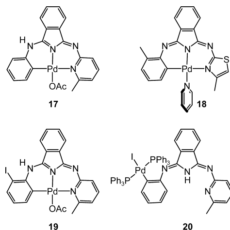
Chart 1. Overview of Palladium(II) Chelates in This Work 17–20
