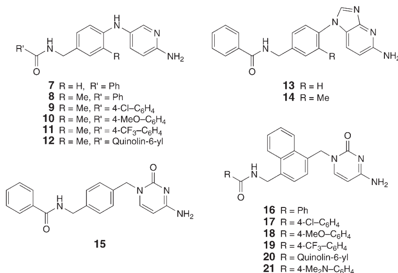
Fig. 1. Cytosine derivatives and analogues prepared as potential inhibitors of IspF
