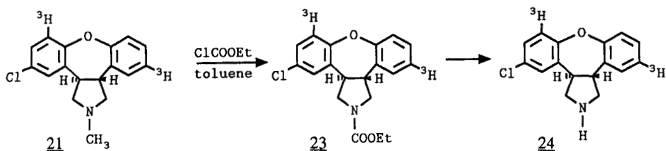
Figure 11: synthesis of [7,11- ^3\text{H} ]-Org 30526
