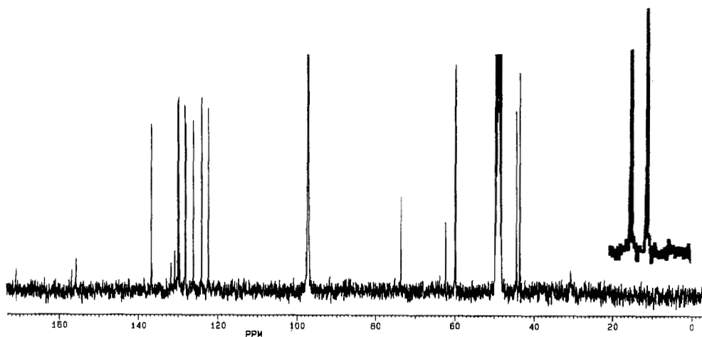
^{13}\text{C} -NMR spectrum of carrier free [12\text{b-}^{14}\text{C}]\text{-Org 5222}
