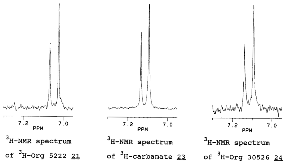
Figure 12: ^3\text{H} -NMR spectra
