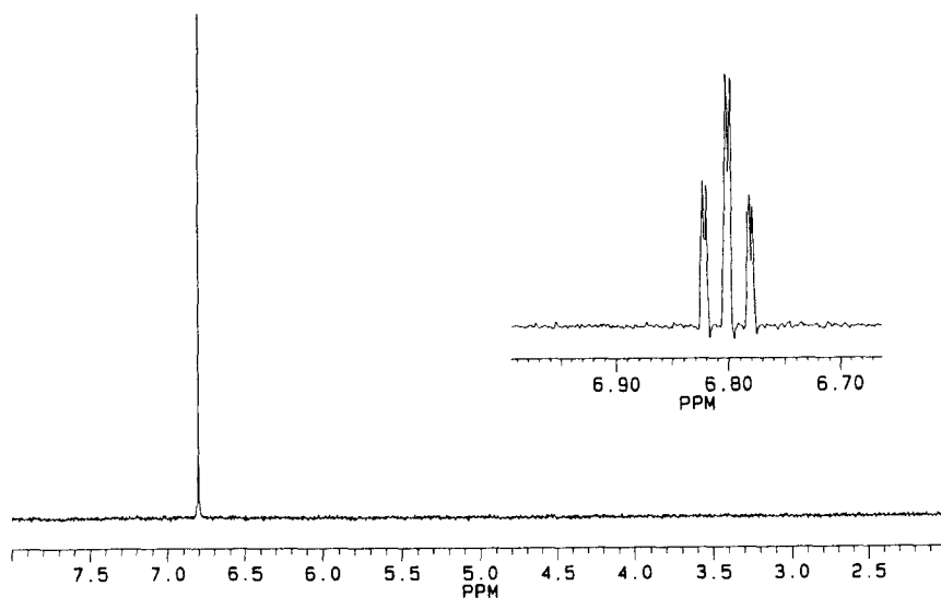
Figure 7: ^3\text{H} -NMR spectra of [11\text{-}^3\text{H}] -Org 5222
