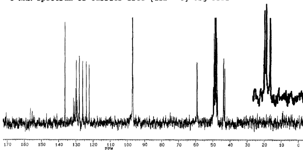
^{13}\text{C} -NMR spectra of [12\text{b-}^{14}\text{C}]\text{-Org 5222} with carrier
