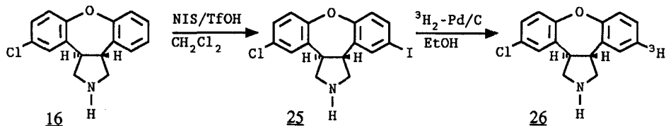
Figure 13: synthesis of [ 11\text{-}^3\text{H} ]-Org 30526
