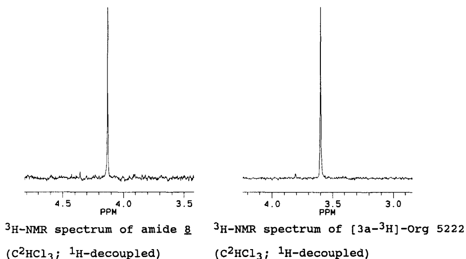
Figure 4: ^3\text{H} -NMR spectra
