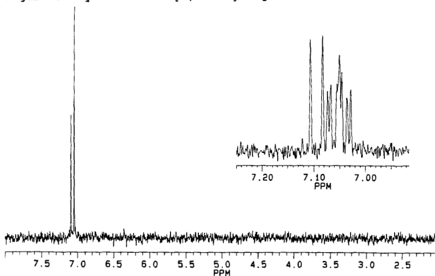
Figure 9: ^3\text{H} -NMR spectra of [7,11- ^3\text{H} ]-Org 5222 ( \text{C}_2\text{HCl}_3 ; ^1\text{H} -decoupled and ^1\text{H} -coupled)
