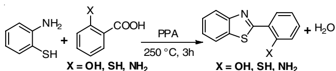
Scheme-I: Synthesis of benzothiazole derivatives
