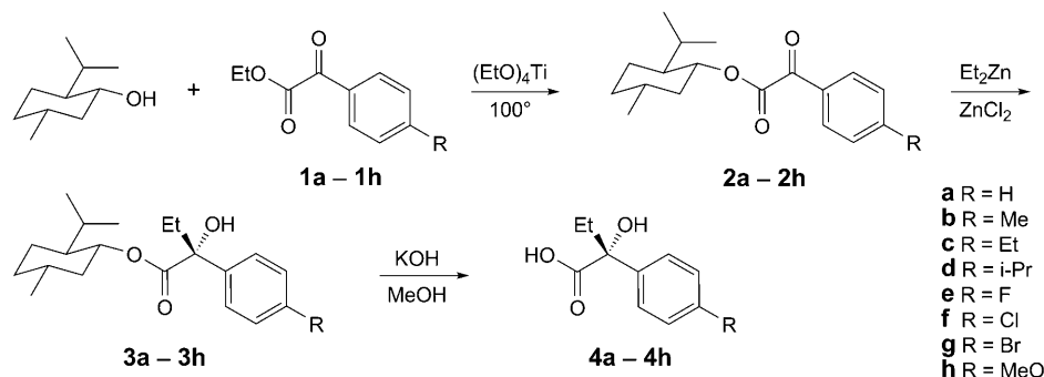
Scheme 1. Synthetic Route to (R)-2-Aryl-2-hydroxybutanoic Acids
