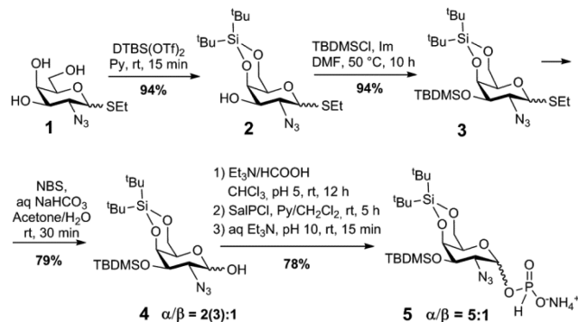
Scheme 1. Synthesis of the Glycosyl-H-phosphonate
